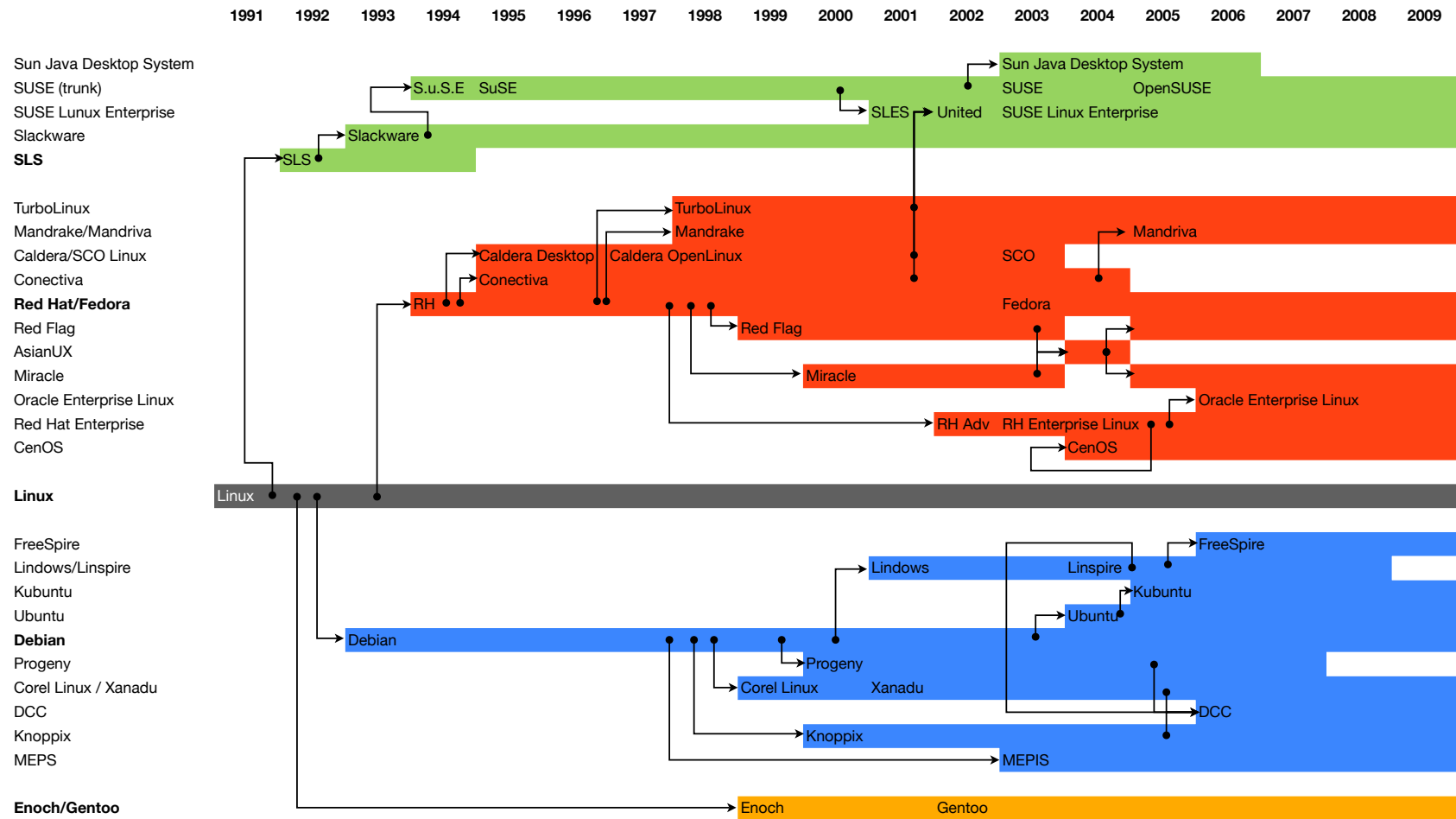
Linux Family Tree. Copyright © Nicholas J. Radcliffe 2009. Based on Ian M. Murdoch's Linux Family Tree ( http://ianmurdoch.com/linux/linux-family-tree-version-0-90/ ). Ian Murdoch's original and this version are both licensed under Creative Commons Attribution 3.0 United States License.
